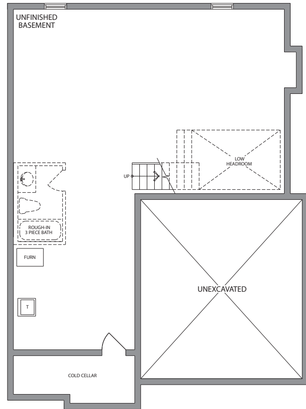
BASEMENT ELEVATION A
