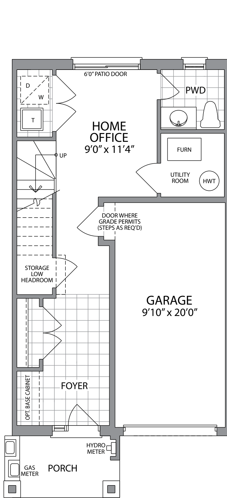
LOWER FLOOR ELEVATION A
