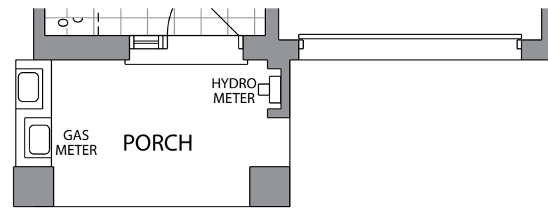
LOWER FLOOR ELEVATION B
