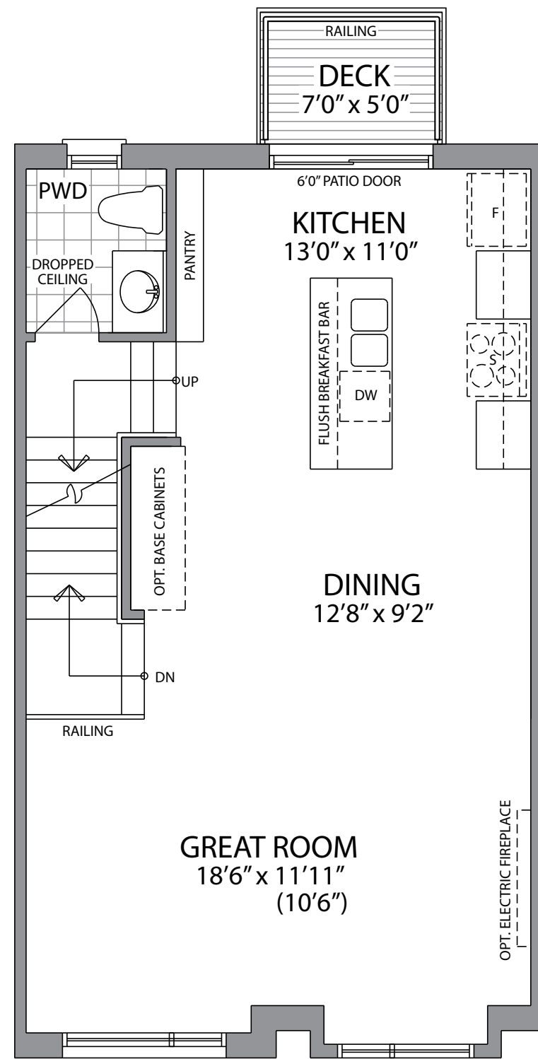
MAIN FLOOR ELEVATION A
