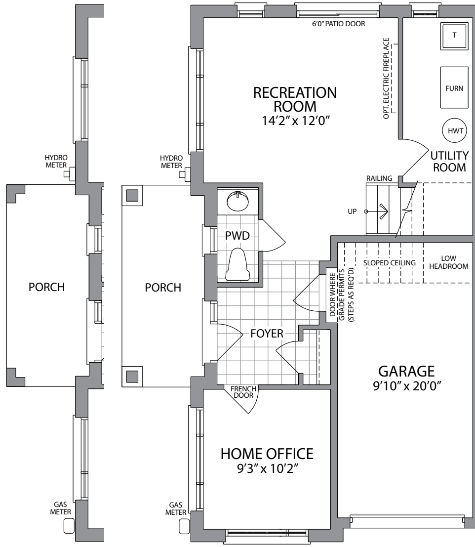
LOWER FLOOR ELEVATION A
