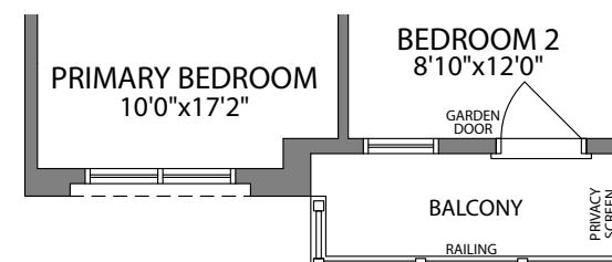
UPPER FLOOR PLAN ELEVATION A2
