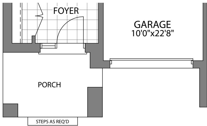
LOWER FLOOR PLAN ELEVATION B
