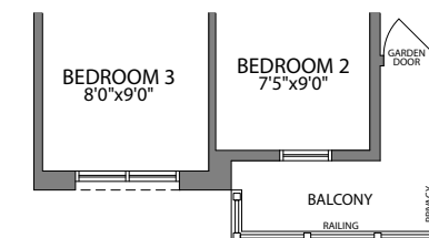
UPPER FLOOR PLAN ELEVATION A2
