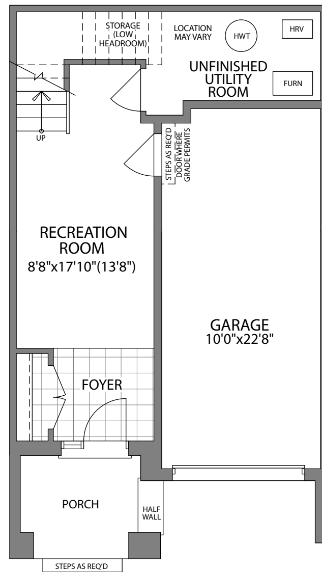
LOWER FLOOR PLAN ELEVATION A1 & A2
