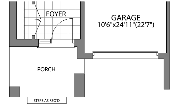
LOWER FLOOR PLAN ELEVATION B
