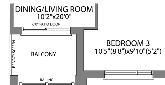
MAIN FLOOR PLAN ELEVATION B1
