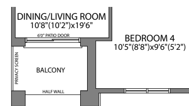
OPT. MAIN FLOOR PLAN ELEVATION A2
