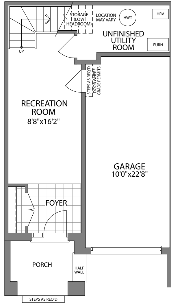
LOWER FLOOR PLAN ELEVATION A1 & A2
