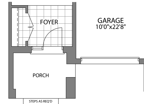
LOWER FLOOR PLAN ELEVATION B1 & B2
