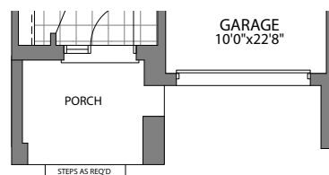
LOWER FLOOR PLAN ELEVATION B1 & B2
