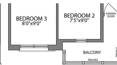
UPPER FLOOR PLAN ELEVATION B1
