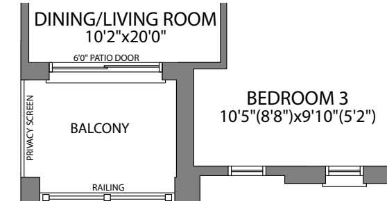
MAIN FLOOR PLAN ELEVATION B2
