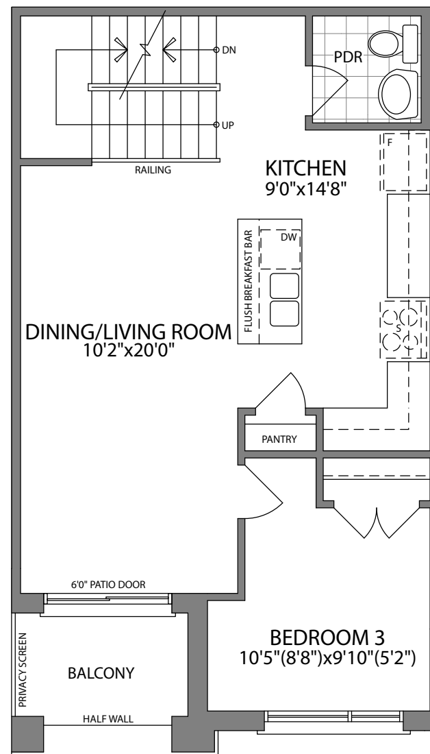
MAIN FLOOR PLAN ELEVATION A1
