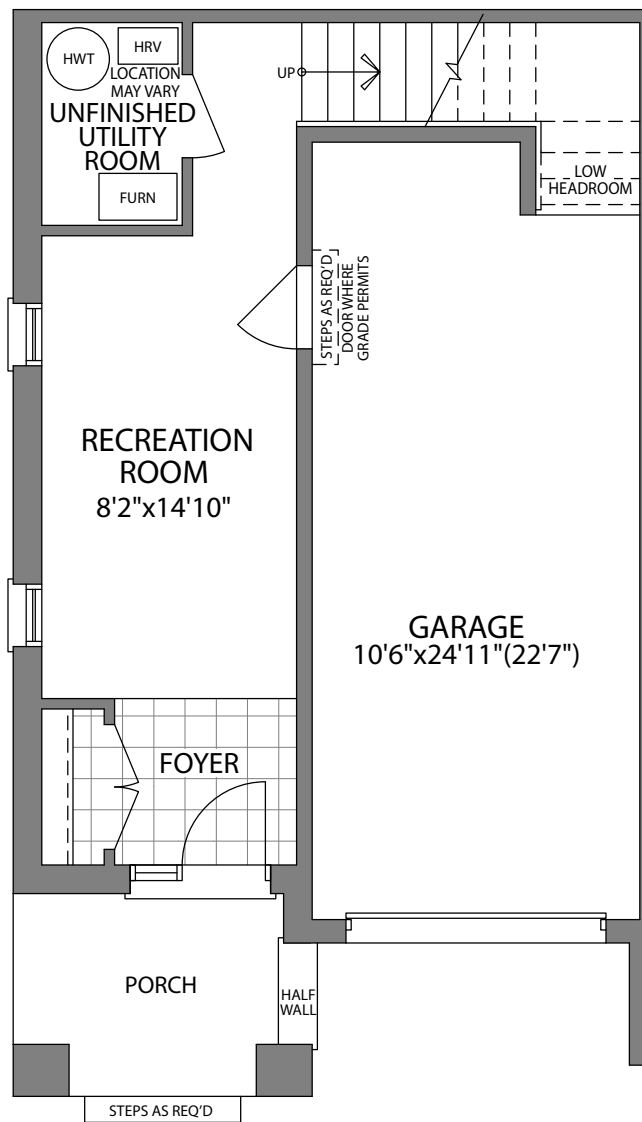
LOWER FLOOR PLAN ELEVATION A
