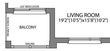
MAIN FLOOR PLAN ELEVATION B1
