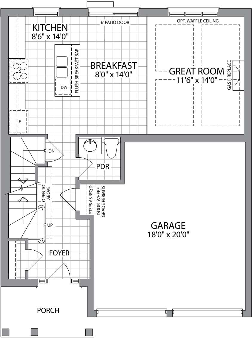
GROUND FLOOR ELEVATION A
